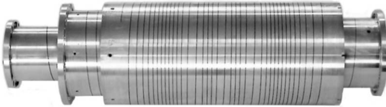
FIG. 7. The four silver layers of a 1 T FFC magnet. The picture shows also a detail of the inner wall of the smallest, most internal layer. The thickness of the cuts is 0.16 mm. At 400 A, the hottest spot power density dissipation reaches 1.1 W/mm 2 . One of the most difficult engineering challenges is to cool these hot spots of the innermost layer efficiently enough to extract all the heat. If the cooling is inefficient, the layer can be seriously damaged or even destroyed.
