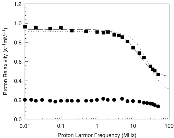
FIG. 14. Paramagnetic enhancements to water ^1\text{H} NMRD profiles for solutions of cobalt(II) human carbonic anhydrase I at pH 9.9 and 298 K (■) (48,49) and for solutions of the nitrate adduct of cobalt(II) bovine carbonic anhydrase II at pH 6.0 and 298 K (●) (126). The dashed line shows the best fit profile of the former data calculated with including the effect of ZFS, whereas the dotted line shows the best fit profile calculated without including the effect of ZFS.
