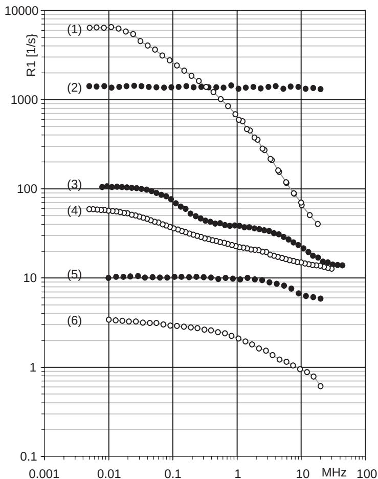
FIG. 29. Examples of FFC NMRD profiles. All NMRD profiles shown here were measured with the Stelar FFC NMR Relaxometer at 25°C using the automated profile acquisition Wizard. The observed nuclide was ^1\text{H} in all cases except (5) where it was ^2\text{D} . The individual curves show: (1) Parafilm M (American National Can Co.), (2) 2.1M \text{Dy}(\text{ClO}_4)_3 in \text{H}_2\text{O} (courtesy Dr.L.Holm), (3) 2mM \text{MnCl}_2 in \text{H}_2\text{O} , (4) egg yolk, (5) 10 mM \text{Gd}^{3+} in \text{D}_2\text{O} , (6) egg albumin.
