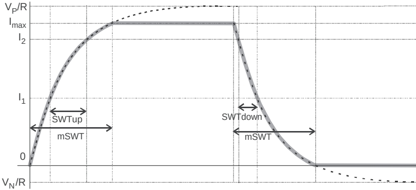
FIG. 13. The fastest current-switching waveform. The diagram shows the magnet current when switching between zero to the maximum admissible current I_{\max} . The horizontal line at V_P/R corresponds to the maximum positive current which a power supply with voltage V_P can deliver into a magnet with resistance R . The line V_N/R defines the extreme negative current which can be generated by the negative power supply section with its extreme negative voltage V_N . The thick curve defines the fastest up- and down-going waveforms, clipped by the imposed limits of 0 and I_{\max} . The two non-stationary sections have a generic exponential form with a time constant given by L/R , where L and R are the inductance and the resistance of the magnet. This defines the absolute minimum switching time mSwT and the fastest-approach waveform. If one wants to actively control the approach, it is necessary to take into account that, at any given current level I , the slope of the actual I(t) curve may not exceed that of the fastest-approach function.
